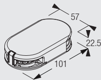
10482 Child Safety device - 4mm Metal Bead Chain
