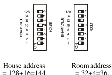
Fig 5. Addressing Switches
