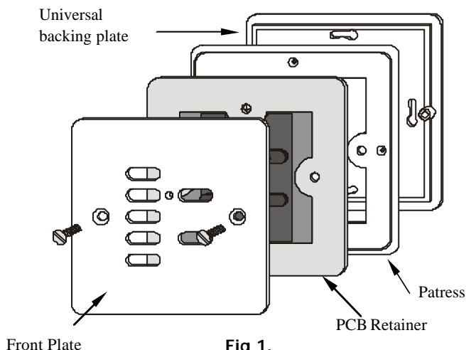
Fig 1. Front View of Components
